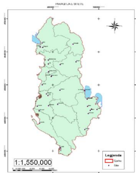
Figure 1. The map of Albania showing the locations where the soil parameters are measured.
