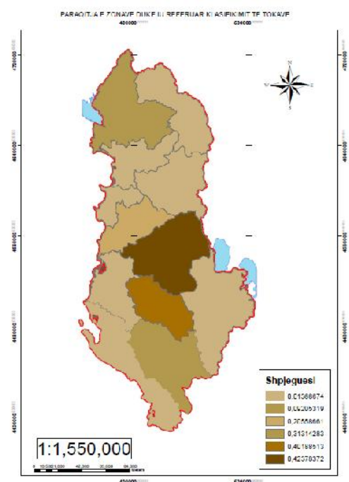
Figure 2. The erodibility map of soils of Albania.
