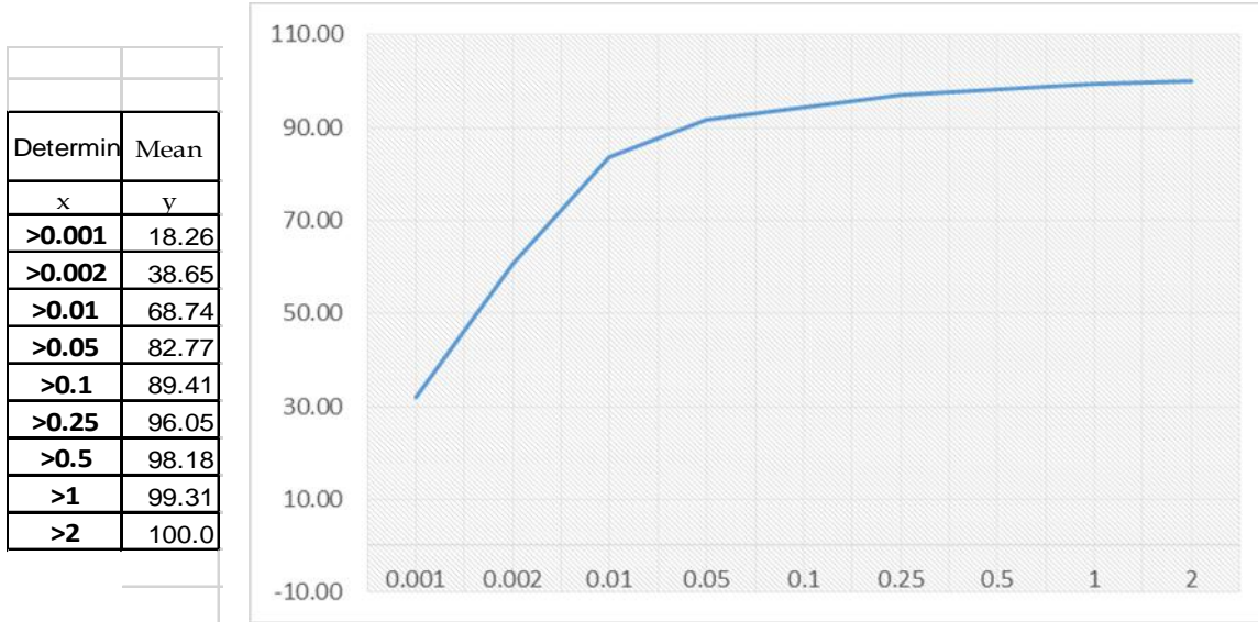
Figure 1. The cumulative particle-size distribution function belonging to Pedon 21, classified as clay
